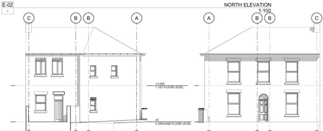
E-02 NORTH ELEVATION 1:100 E-03 EAST ELEVATION 1:100 E-01 WEST ELEVATION 1:100
